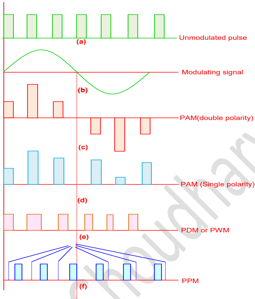
Different types of pulse modulated signals
